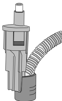
Mr. Drain and washing machine hose in 1-1/2" plastic standpipe .
