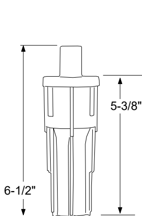
Fig.1 Dimensions
